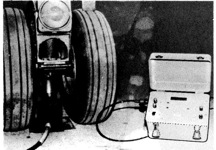
“ROAD RUNNER” II WEIGHING 737 AIRCRAFT
