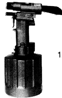
MODEL 200 1/8" through 1/4" rivet capacity 5/32" through 1/4" bolt cap.
